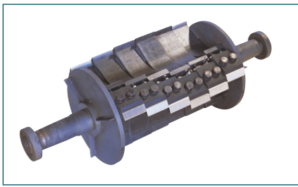
Claw Type Cutterhead
