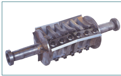
Bevel Type Cutterhead
